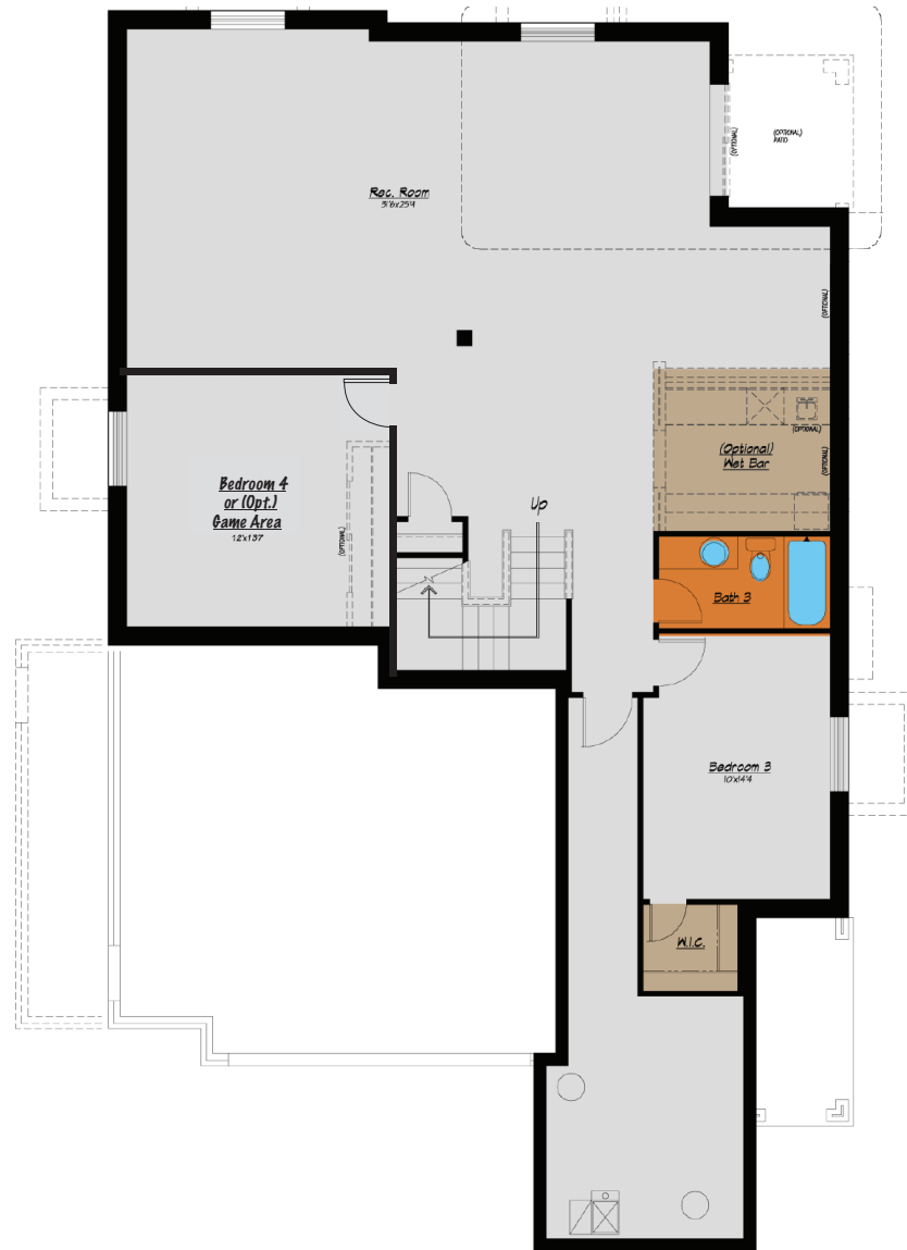
BASEMENT LEVEL
